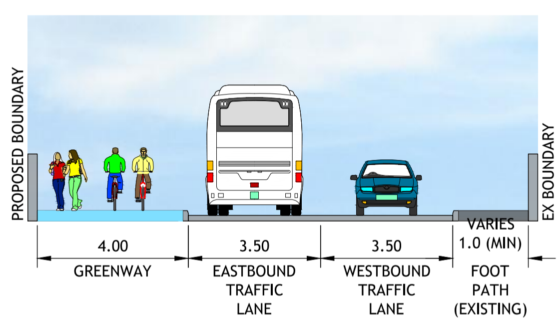
TYPICAL CROSS SECTION TYPE A-1 (CH 0 TO 600)
