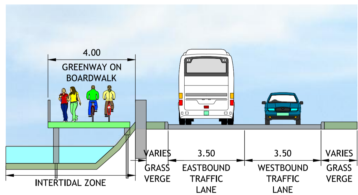
TYPICAL CROSS SECTION TYPE D-2 (CH 2000-2100)
