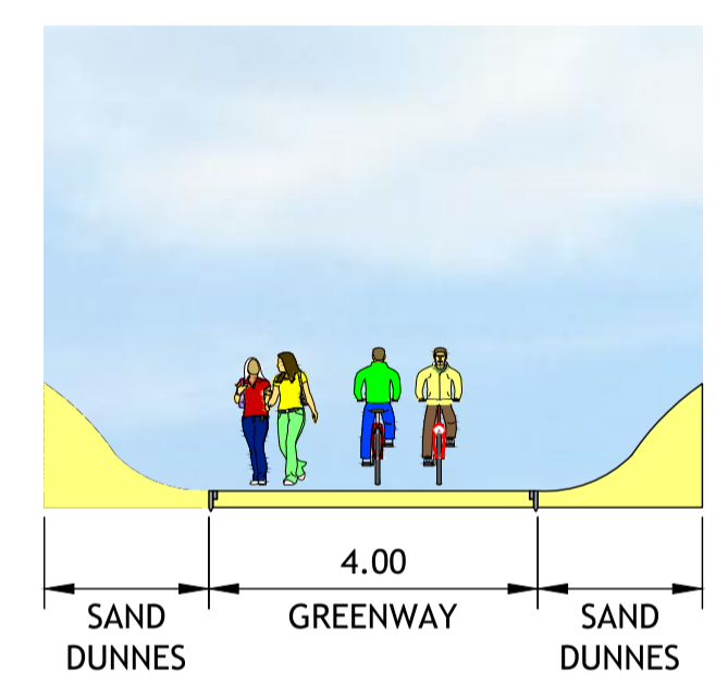
TYPICAL CROSS SECTION TYPE C (CH 5890-6445)
