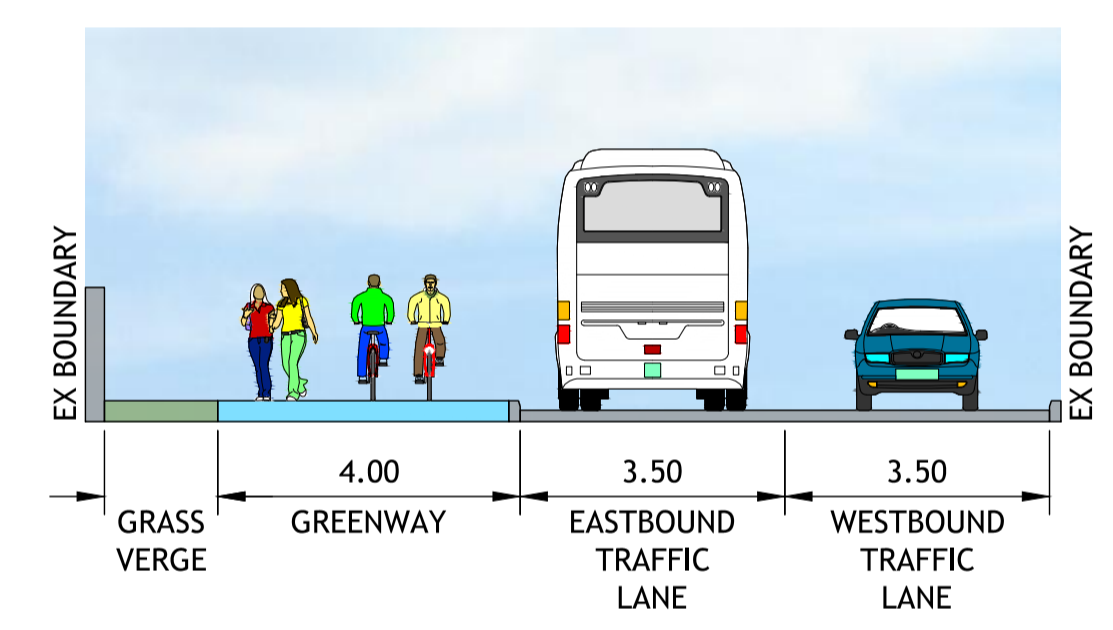
TYPICAL CROSS SECTION TYPE A-1 (CH 600 TO CH 740)
