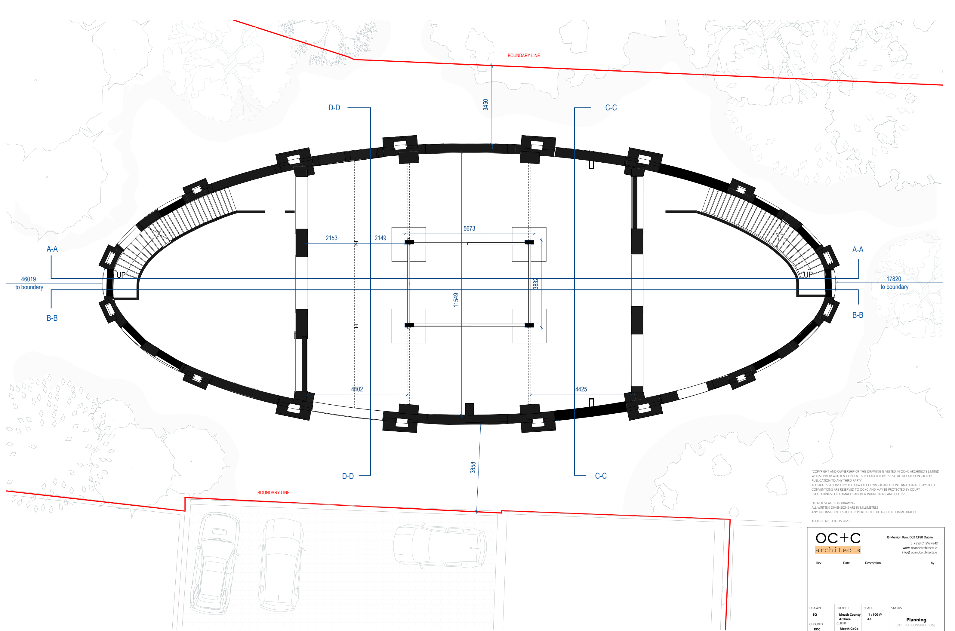
1 Ground Floor Plan (Existing) Scale - 1 : 100
