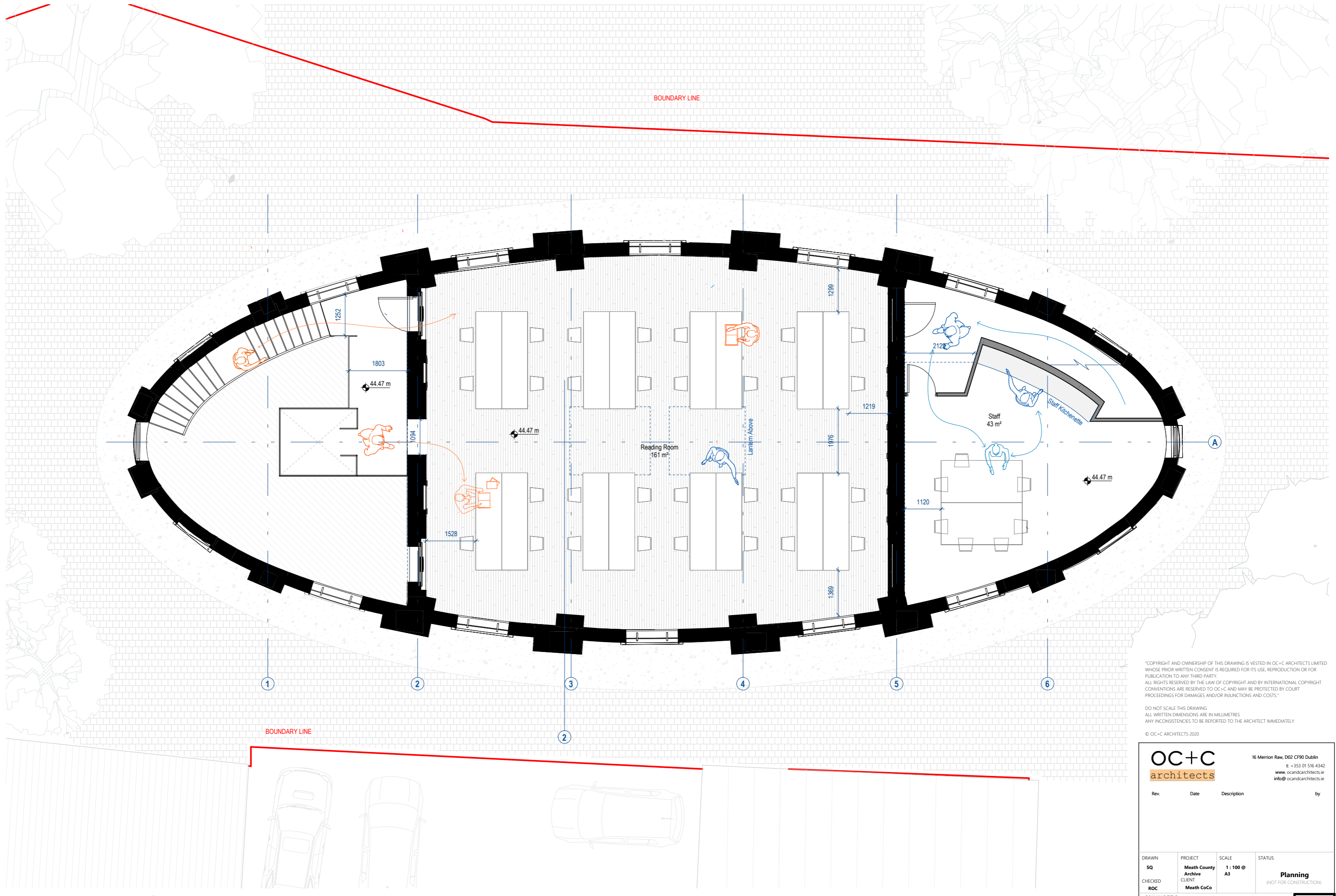
1 First Floor Plan Scale - 1:100
