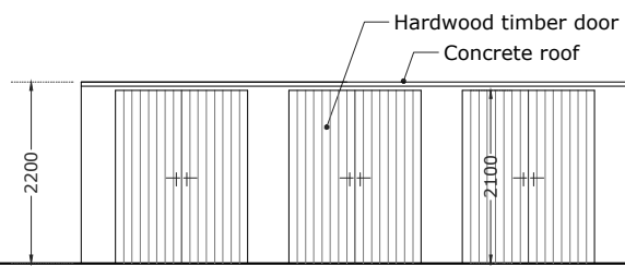
Proposed Bin Store Elevations Scale 1:100
