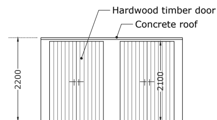
Proposed Bicycle Store Front Elevations Scale 1:100
