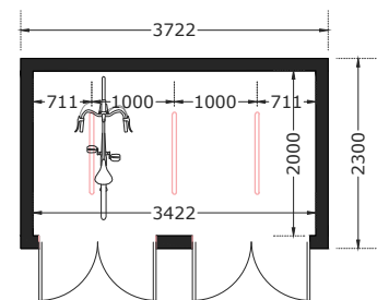
Proposed Bicycle Store Plan Scale 1:100
