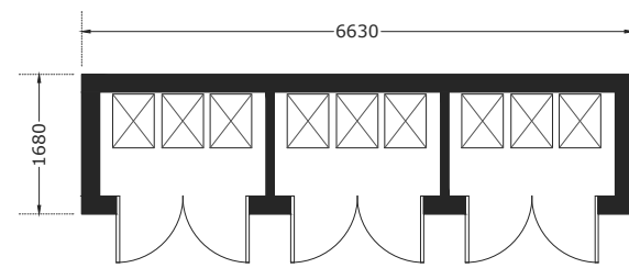
Proposed Bin Store Plan Scale 1:100
