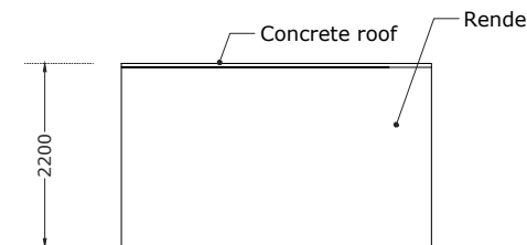
Proposed Bicycle Store Rear Elevations Scale 1:100
