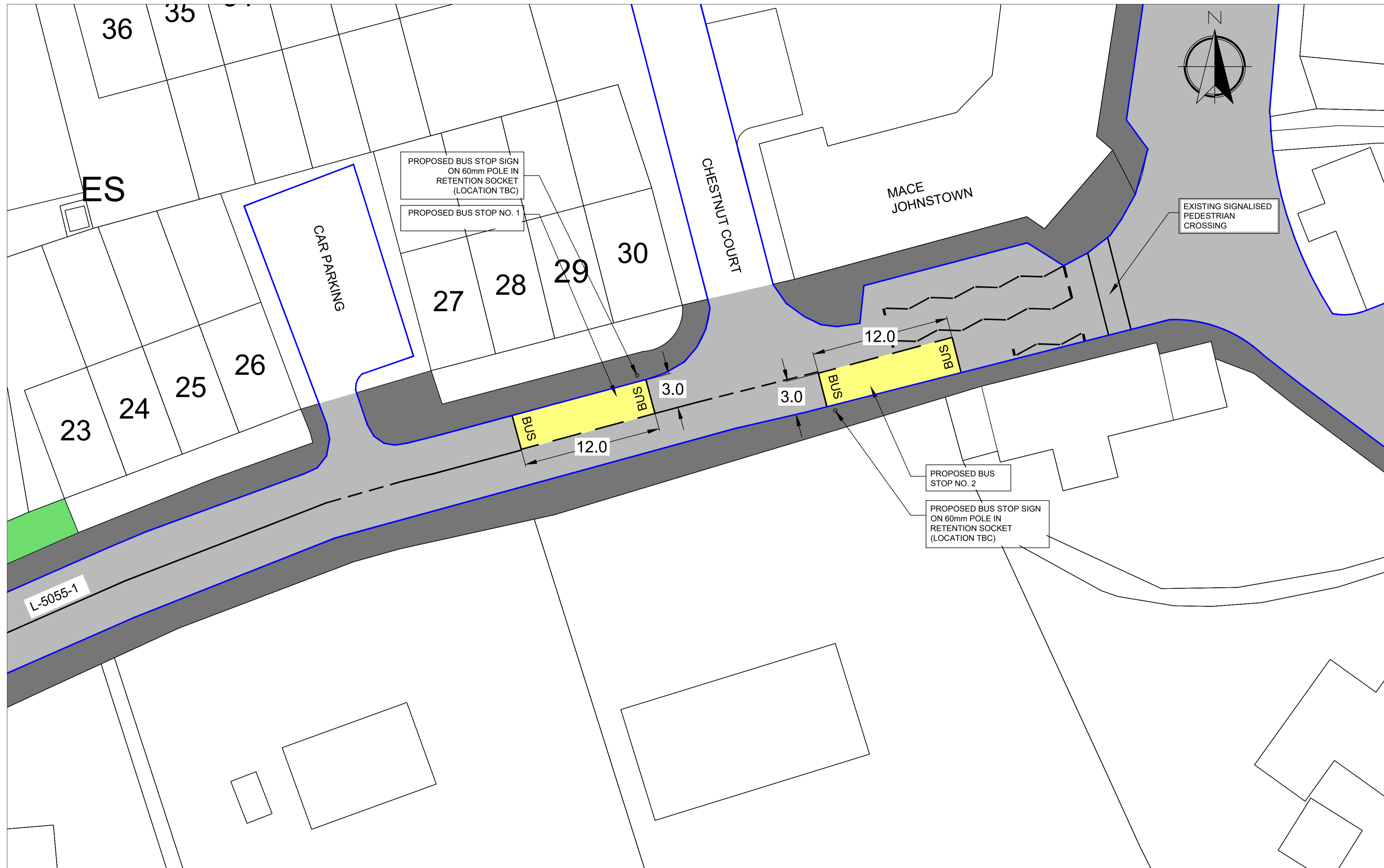
PROPOSED IN-LINE BUS STOPS NO. 1 & 2
