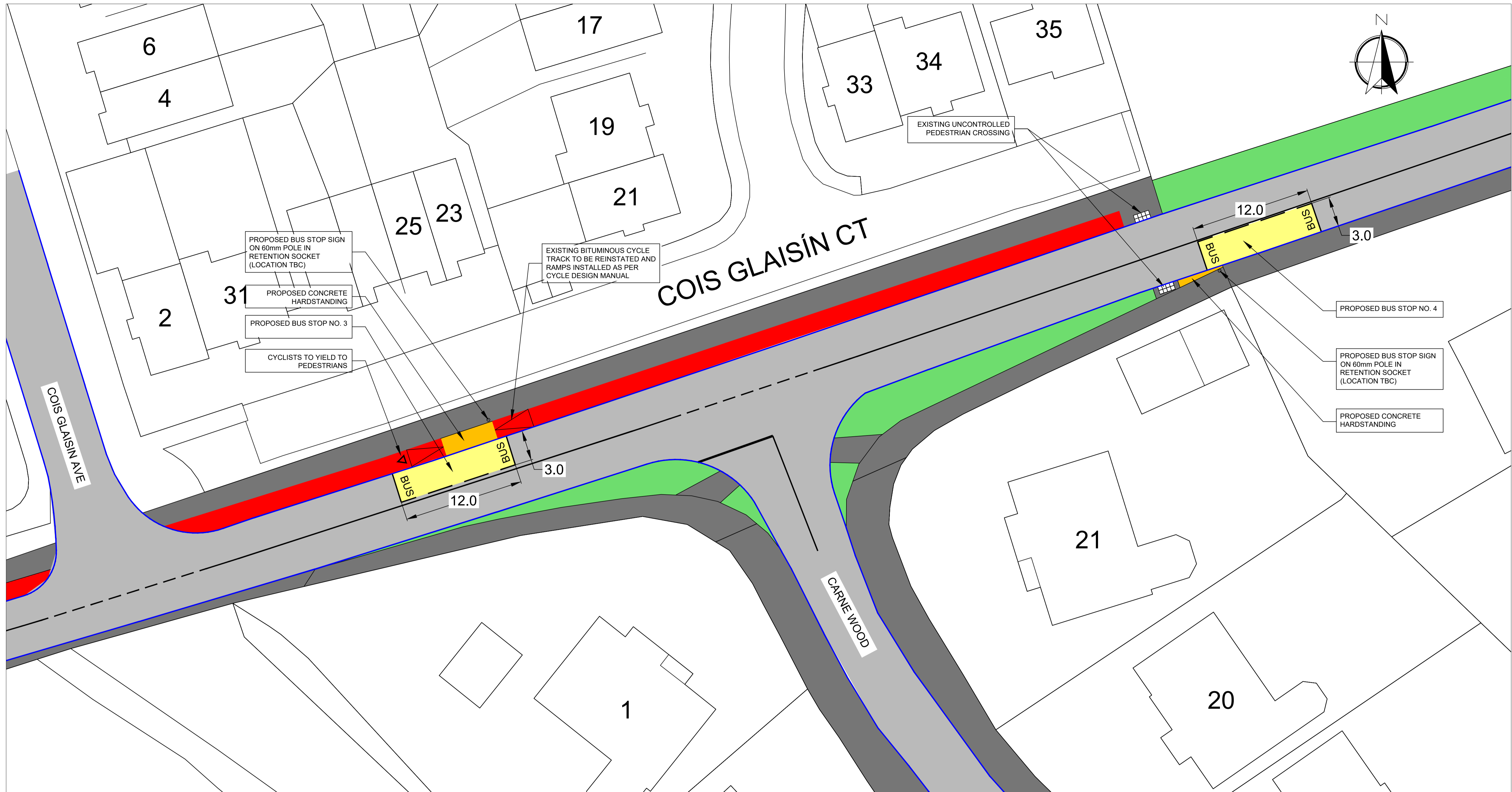
PROPOSED IN-LINE BUS STOPS NO. 3 & 4
