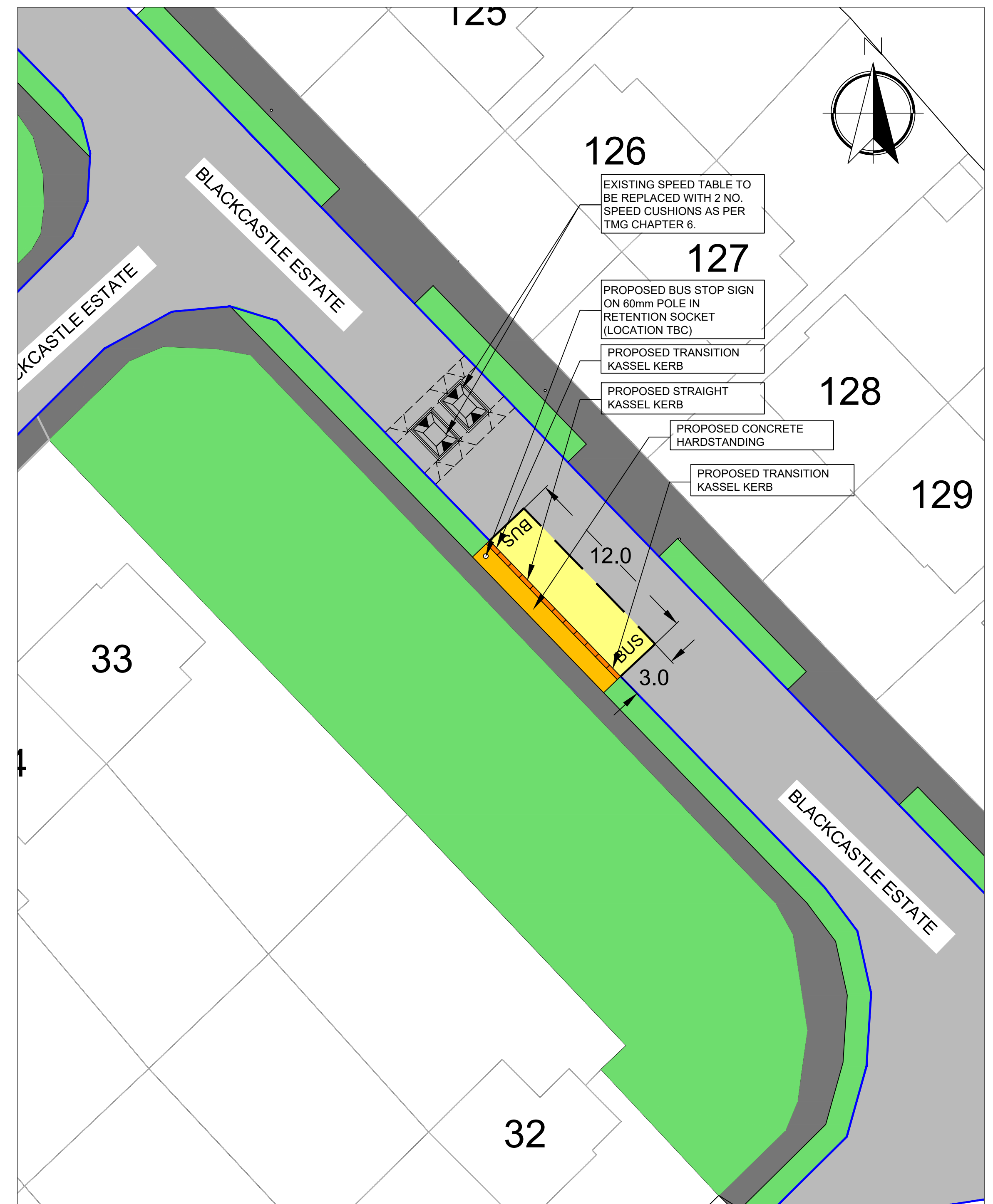
PROPOSED IN-LINE BUS STOP NO. 7
