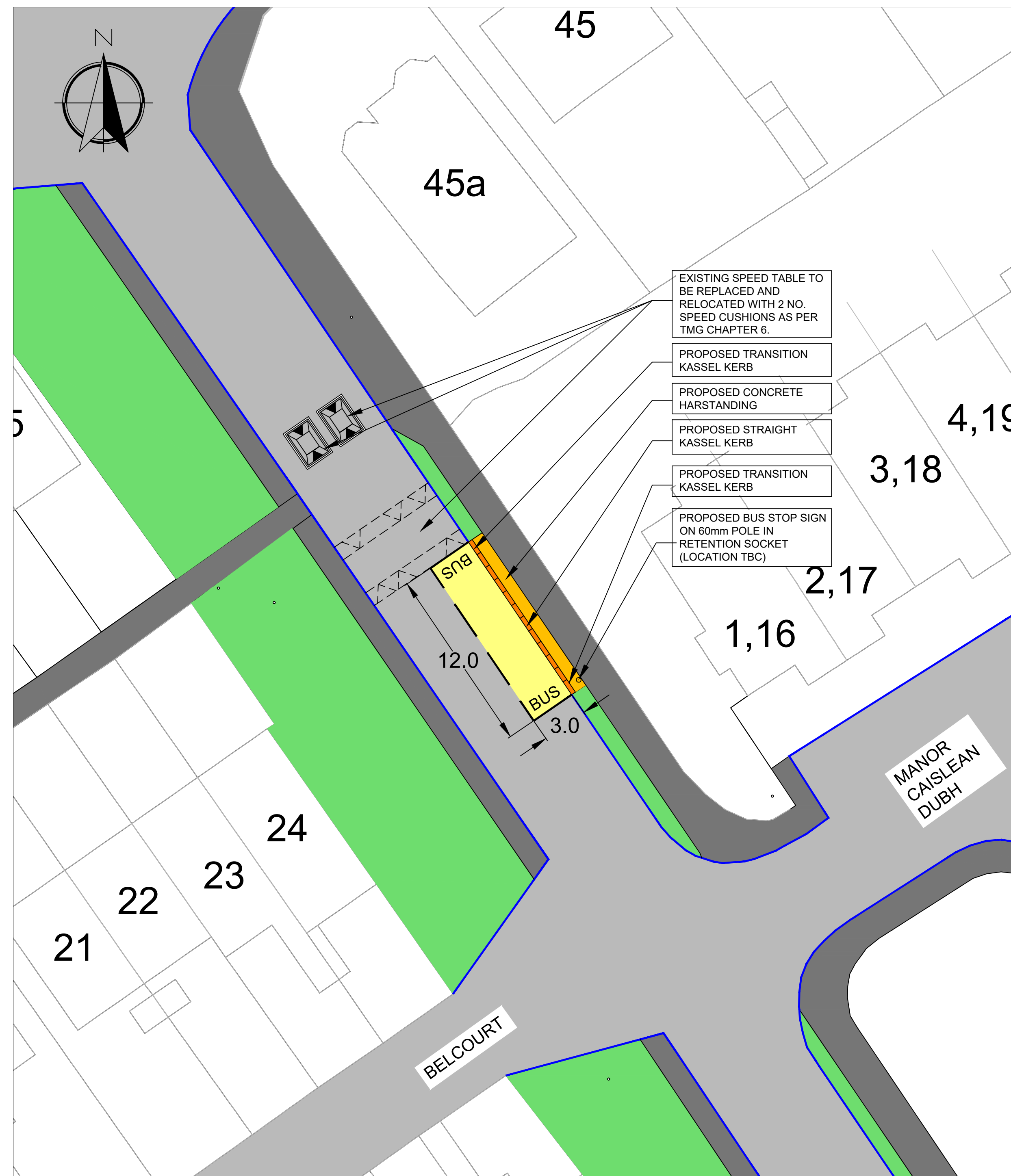
PROPOSED IN-LINE BUS STOP NO. 6
