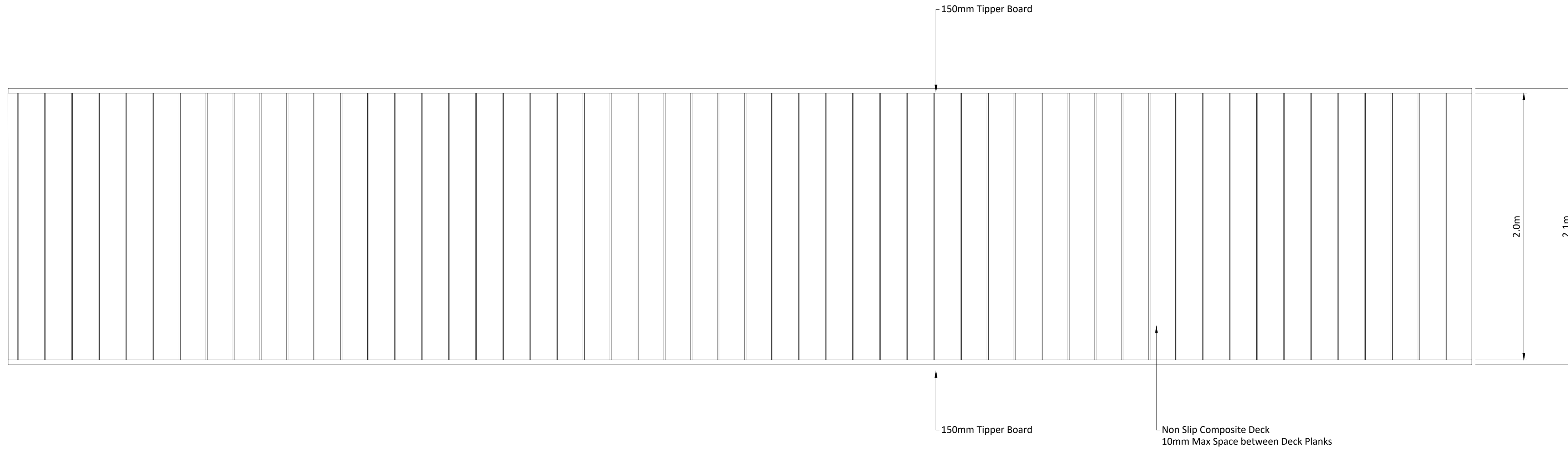
TYPICAL JETTY DETAIL PLAN Scale 1:20
