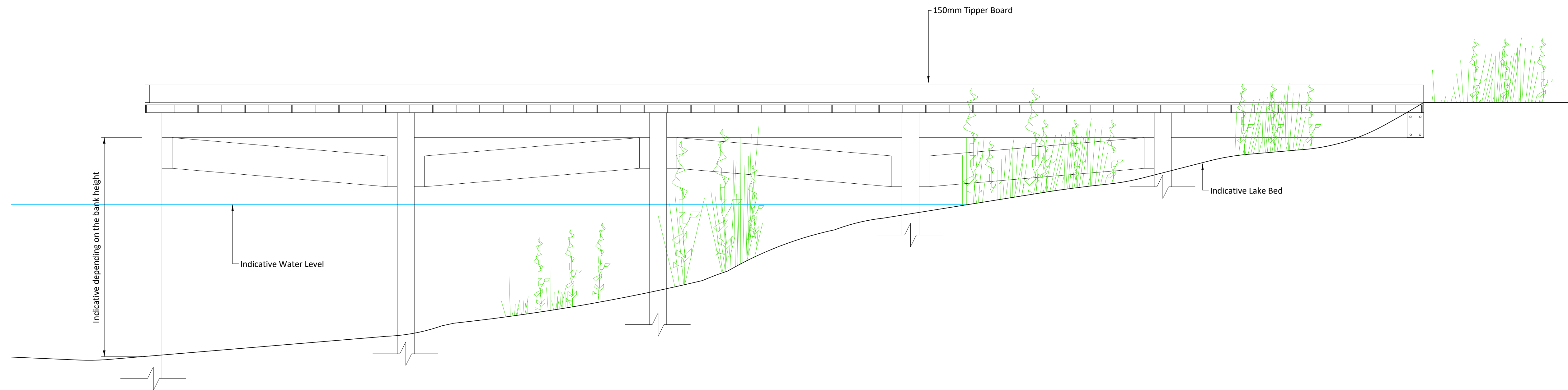
TYPICAL JETTY DETAIL ELEVATION Scale 1:20
