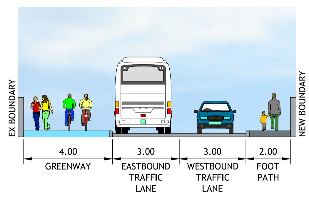
TYPICAL CROSS SECTION TYPE A-4 (CH 5250-CH 5320)
