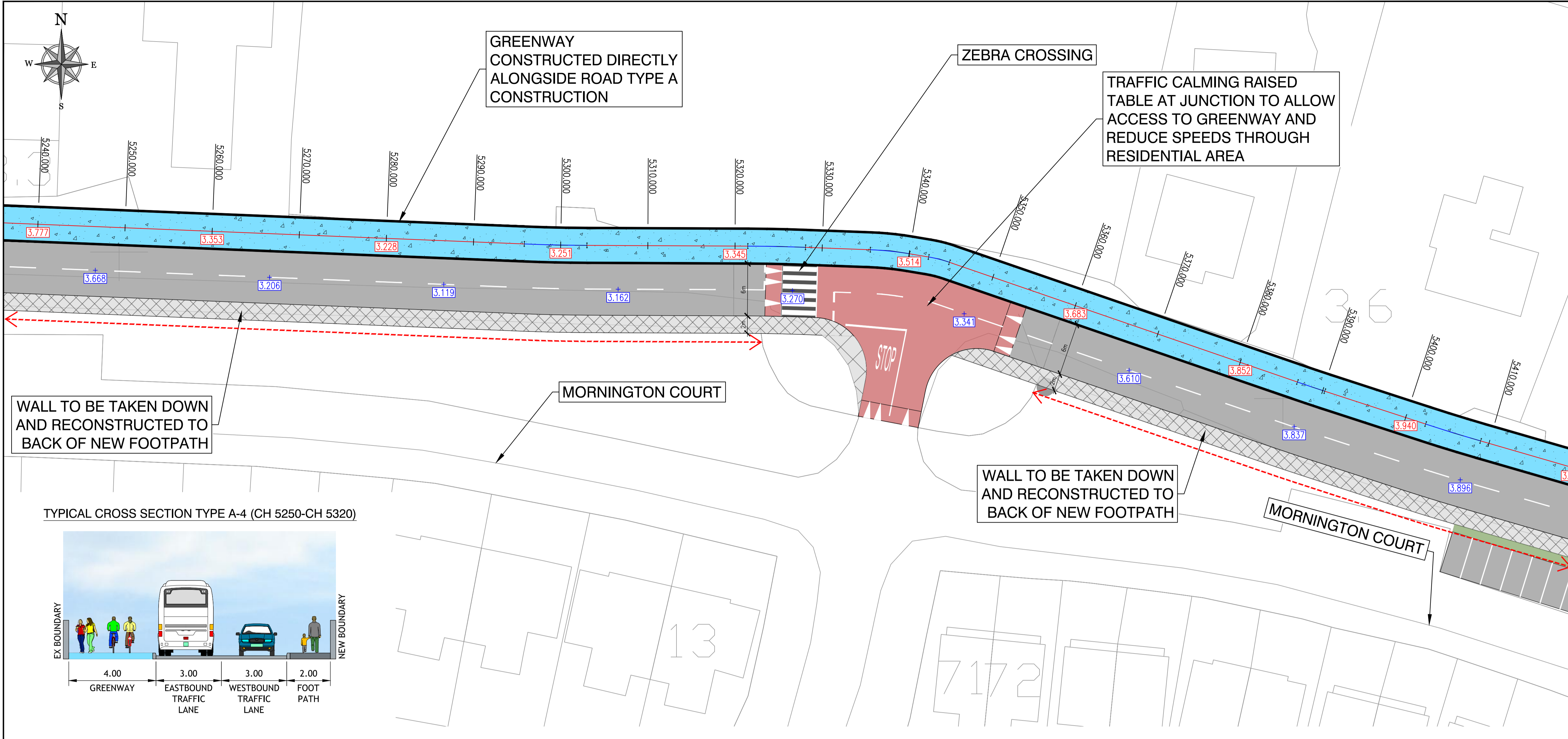
KEYPLAN
