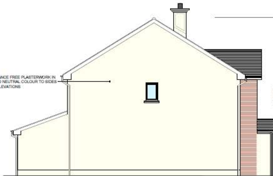
SIDE ELEVATION (TYPICAL)
