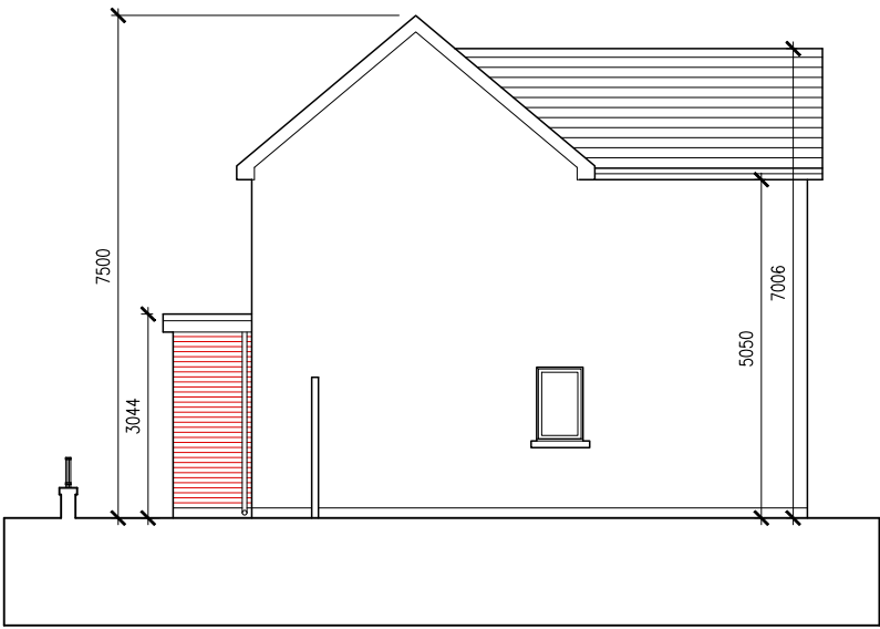
NORTH ELEVATION
